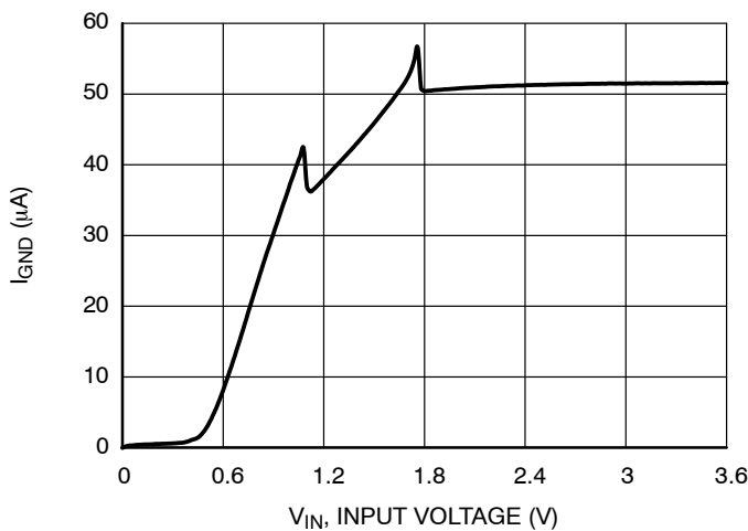
Figure 13. Supply Current vs. Input Voltage, 1.2 V Version
